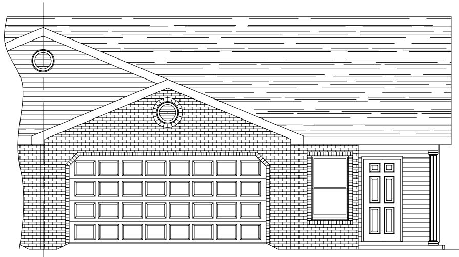
ELEVATION "B"
