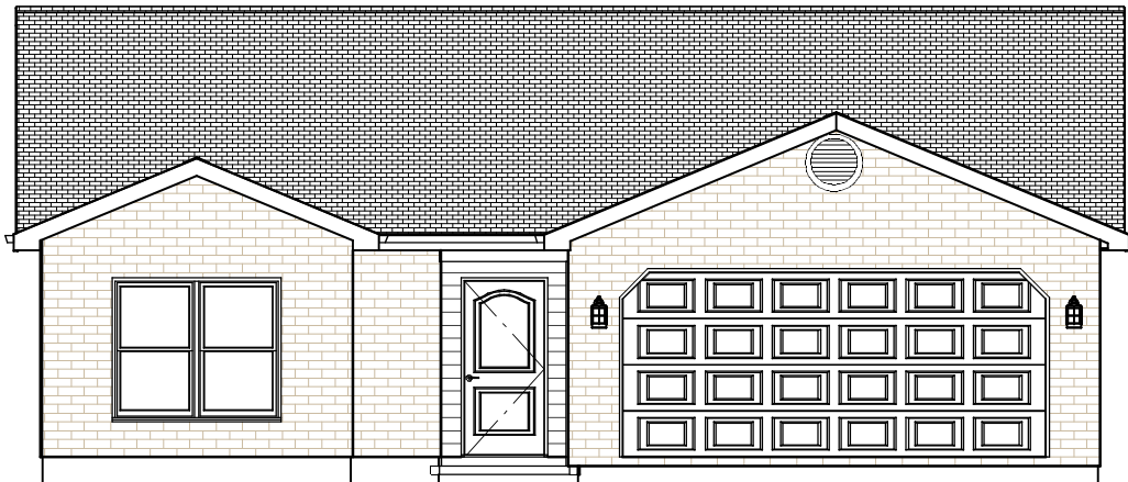
FRONT ELEVATION A SHOWN WITH OPTIONAL FULL BRICK
