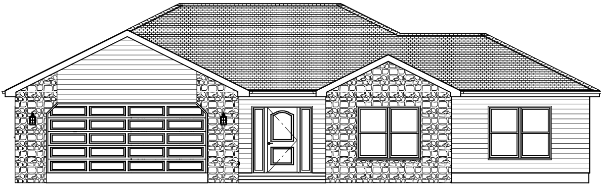
ELEVATION "B" (SHOWN WITH OPTIONAL SIDELIGHTS AND STONE)
