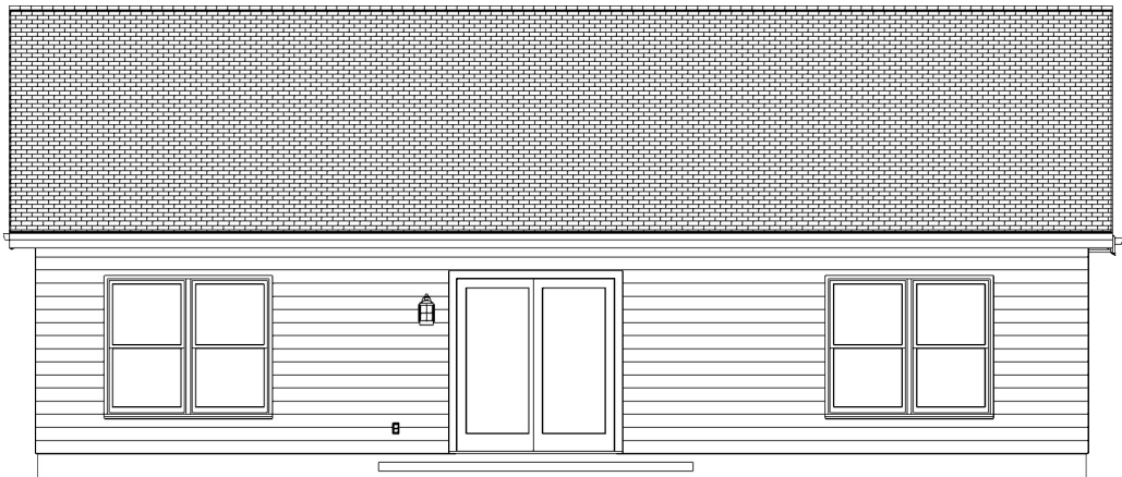
REAR ELEVATION
