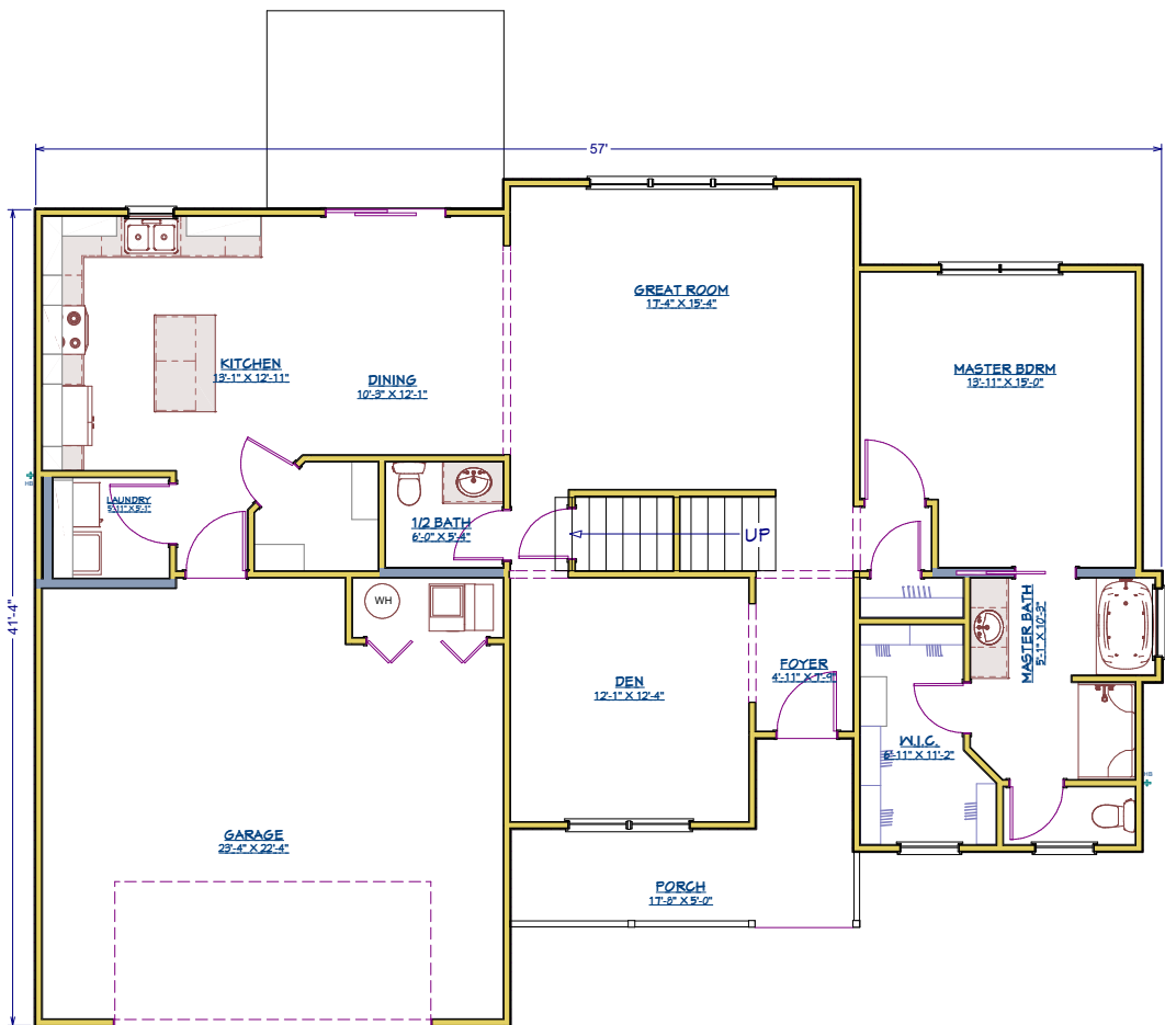
MAIN FLOOR
