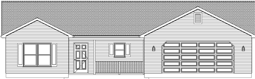
ELEVATION "A"
