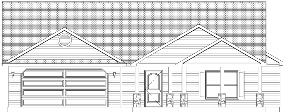
FRONT ELEVATION BOOKLYN C
