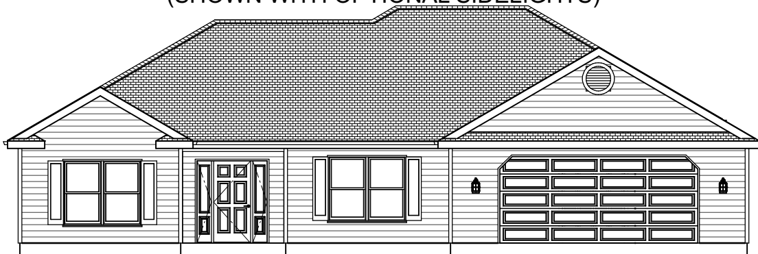
ELEVATION "B" (SHOWN WITH OPTIONAL SIDELIGHTS)
