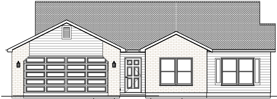
ELEVATION A WITH PARTIAL BRICK
